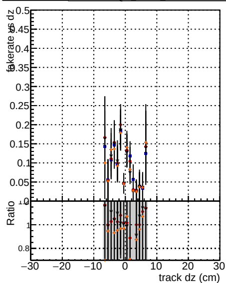
Fake rate vs dz Legend: DSM mkFit T-Original-106 DSM mkFit T-NEWHSM95-ALLITERS-106 DSM mkFit T-NEWHSM95-ALLITERS-106
