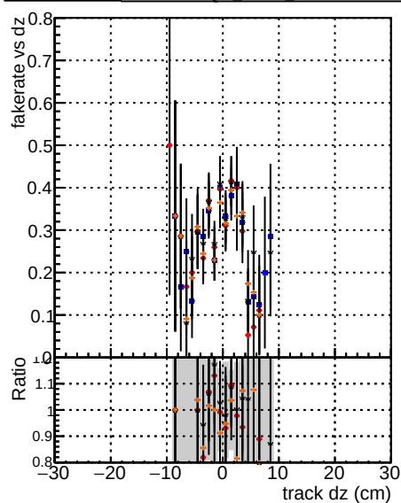
Fake rate vs dz Legend: DSM mkFit T-Original-106 DSM mkFit T-NEWHSM95-ALLITERS-106
