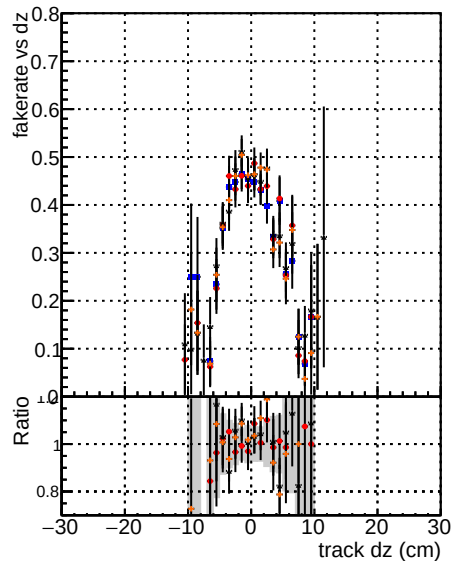
Fake rate vs dz Legend: BQM mktFit (blue), T-Original (red), T-NEW (orange), T-NEWMS95 (green), ALLITERS-106 (black), ALLITERS-95 (grey), ALLITERS-106 (black), ALLITERS-95 (grey)
