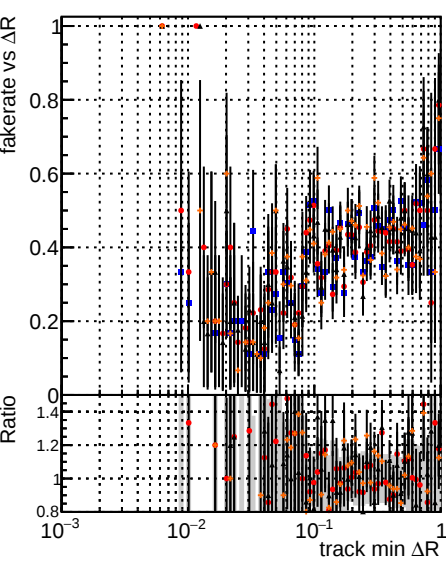
Fake rate vs \Delta R (track, jet) Legend: DOM, mktFit, Original, NEWHSMS95, ALLITERS-106
