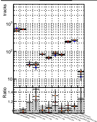
N of reco track vs. \chi^2 for original vs. BGM, mFit, TFit, NEWFSM, ALLITERS-106
