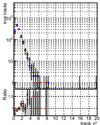
N of reco track vs. \chi^2 for original vs. BGM, mFit, TFit, NEWFSM, ALLITERS-106
