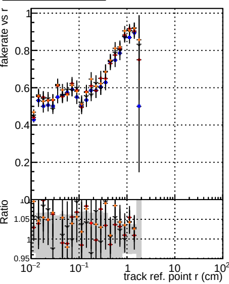
Fake rate vs v DOM mkFit Toriginal DOM mkFit Toriginal-106 DOM mkFit TNEWHSMS95 ALLITERS-106
