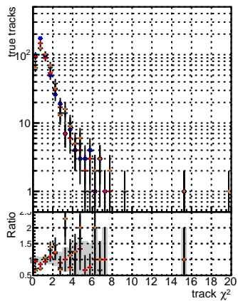
N of reco track vs. \chi^2 for BGM, mFit, TITANUS, and ALLITERS-106
