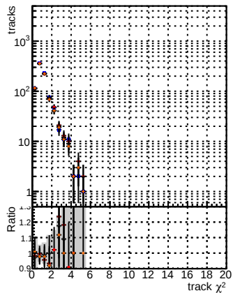
N of reco track vs. \chi^2 BSM mFEL TITAN Original
