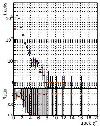
N of reco track vs. \chi^2 for BSM mFEL + T + S + L + S, BSM mFEL + T + S + L, BSM mFEL + T + S, BSM mFEL + T, and BSM mFEL
