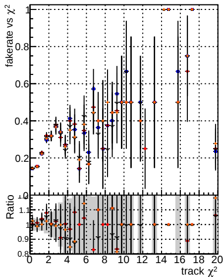
Fake rate vs. BOM mKEit TToriginal TTNEW WFSM106 WFSM95 ALLITERS106
