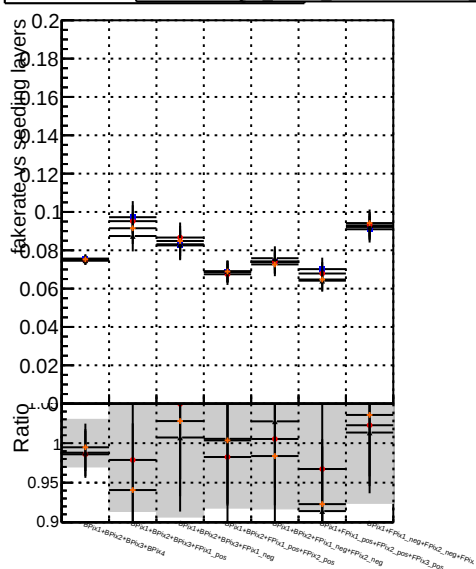
Fake rate vs. seedling layers Legend: BQM mkFit, T-Original, BQM mkFit, T-NEWHSM
