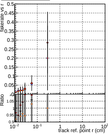
Fake rate vs v DOM mkrFit Toriginal DOM mkrFit Tnew DOM mkrFit TNEW 106 106 106 95 ALLITERS-106
