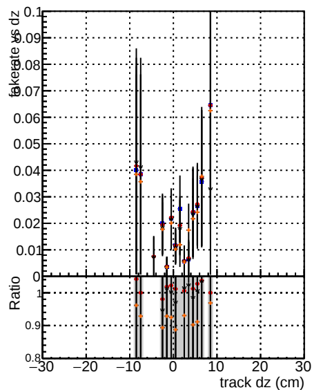
Fake rate vs dz Legend: DOM mkFit Toriginal 106, DOM mkFit TNEWHSMS95, DOM mkFit TALLITERS106
