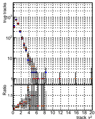
N of reco track vs. \chi^2 BSM mFit TFit Original
