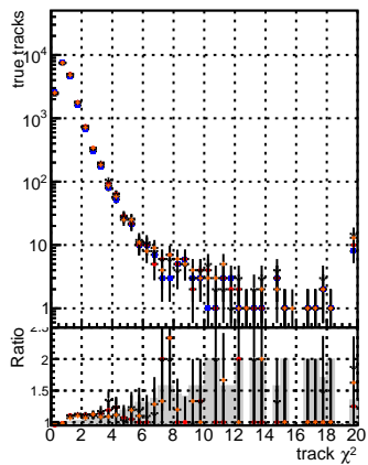
N of reco track vs. \chi^2 for BGM, mFit, and Original tracks
