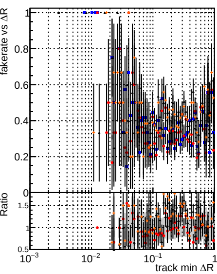
Fake rate vs \Delta R(\text{track, jet}) Legend: DOM (black), mktFit (blue), Toriginal (red), NEWHSMS95 (orange), ALLTERS-106 (green)
