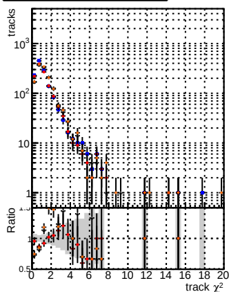
N of reco track vs. \chi^2 for BSM mFit (blue circles), BSM mFit (orange squares), and BSM mFit (red triangles). The x-axis is track \chi^2 and the y-axis is the number of tracks. The bottom panel shows the ratio of tracks.
