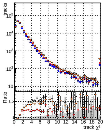
N of reco track vs. \chi^2 for BSM, mFit, Traditional, and ALLITERS-106
