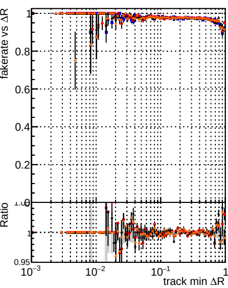
Fake rate vs \Delta R(\text{track, jet}) Legend: DOM (black line with circles), mkFit (blue line with circles), Toriginal (red line with circles), TNEW (orange line with circles), TNEW-SMS95 (green line with circles), TNEW-SMS95-ALLITERS-106 (purple line with circles).
