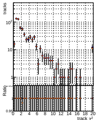
N of reco track vs. \chi^2 for BSM models: Original vs. BSM model: NEWSM95 ALLITERS-106
