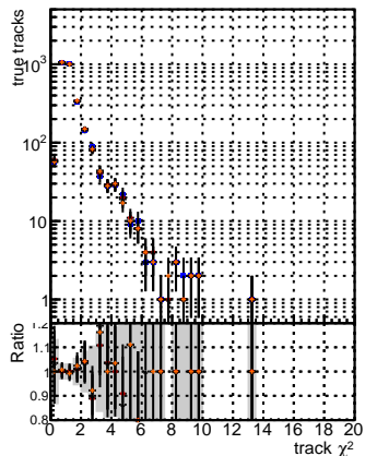
N of reco track vs. \chi^2 for BGM, mFit, Trivial, and NEWFSM95-ALLITERS-106
