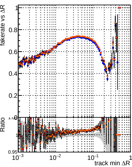
Fake rate vs \Delta R(\text{track, jet}) Legend: DOM mkFit Toriginal-106 DOM mkFit Toriginal-106 DOM mkFit TNEWHSMS95 ALLTERS-106
