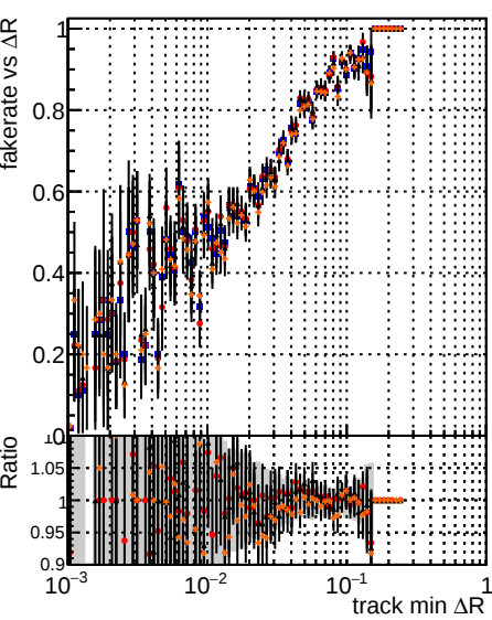
Fake rate vs \Delta R(\text{track, jet}) Legend: DOM, mkFit, Toriginal, TNEW, S95, ALLITERS-106
