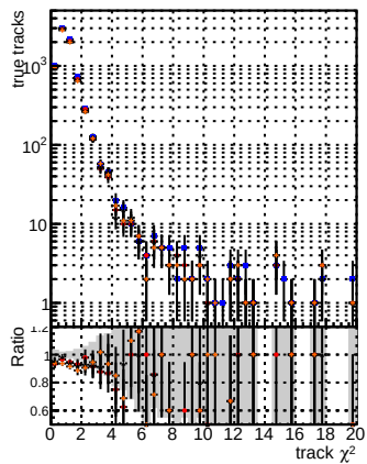
N of reco track vs. \chi^2 for BSM mFEL, BSM mFEL NEWISM95, and BSM mFEL ALLITERS-106
