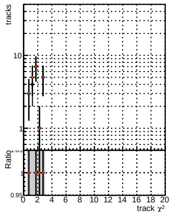
N of reco track vs. \chi^2 for BSM mFit + Traditional vs BSM mFit + NEWISM95 ALLITERS-106
