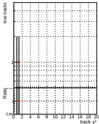
N of reco track vs. \chi^2 for BSM mFit + Traditional vs BSM mFit + NEWISM95 ALLITERS-106
