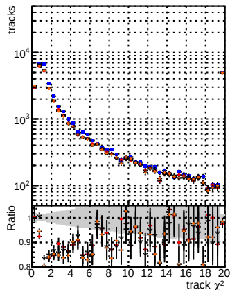
N of reco track vs. \chi^2 for BSM model TToriginal-05, BSM model TTNEWISM-95, and ALLITERS-106
