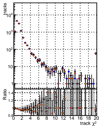
N of reco track vs. \chi^2 for BSM mFit + Original vs BSM mFit + NEWFSM95 vs ALLITERS-106
