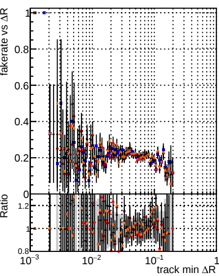
Fake rate vs \Delta R(\text{track, jet}) Legend: DOM (black), mkFit (blue), T-Original (red), T-New (orange), T-New-S95 (grey), ALLITERS-106 (black), ALLITERS-106 (red), ALLITERS-106 (orange), ALLITERS-106 (blue).
