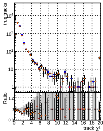
N of reco track vs. \chi^2 for BSM mFit + Traditional vs BSM mFit + NEW
