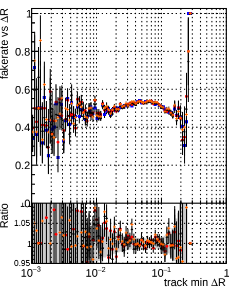
Fake rate vs \Delta R(\text{track, jet}) Legend: DOM mkFit Toriginal-106, DOM mkFit Toriginal-106, DOM mkFit TNEWHSMS95 ALLITERS-106
