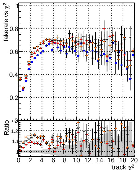
Fake rate vs. BQM mkFit T-Original 106 BQM mkFit T-NEWHSMS95 ALLITERS-106
