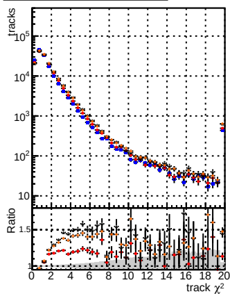
N of reco track vs. \chi^2 BSM mFit TFit TFit ALLITERS-106
