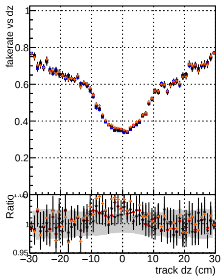
Fake rate vs dz DQM mkFit T (original) 106 DQM mkFit T (NEWS) 95 DQM mkFit T (ALLITERS) 106
