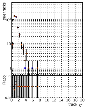
N of reco track vs. \chi^2 for different models
