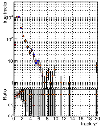
N of reco track vs. \chi^2 BSM mFit TFit Original vs BSM mFit TFit NEWHSMS95 ALLITERS-106
