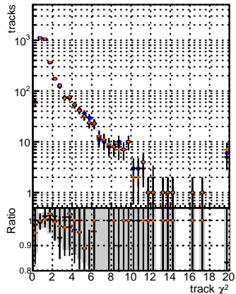
N of reco track vs. \chi^2 BSM mFit TFit Original vs BSM mFit TFit NEWHSMS95 ALLITERS-106
