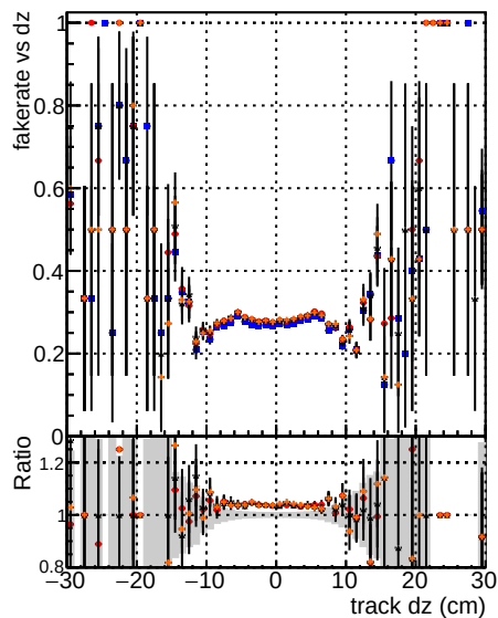
Fake rate vs dz DGM mkFit T-Original DGM mkFit T-NEW HSM95 ALLITERS-106
