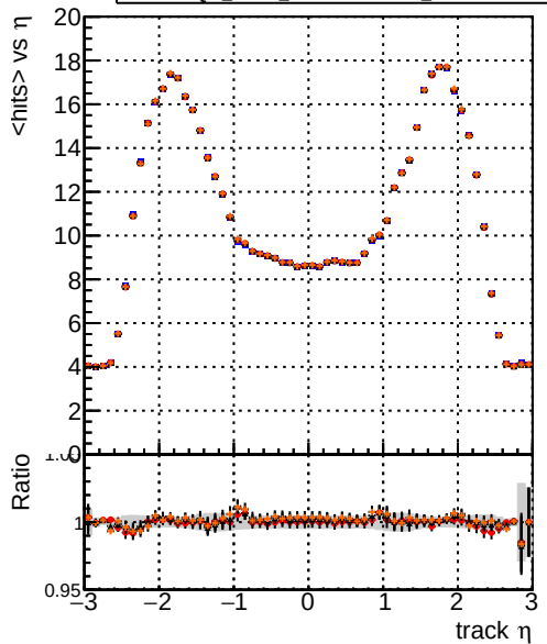
— DQM_mkFit_TToriginal — DQM_mkFit_TToriginal-106 — DQM_mkFit_TTNEWHSMS95_ALLITERS-106 — DQM_mkFit_TTNEWHSMS90_ALLITERS-106 mean hits
