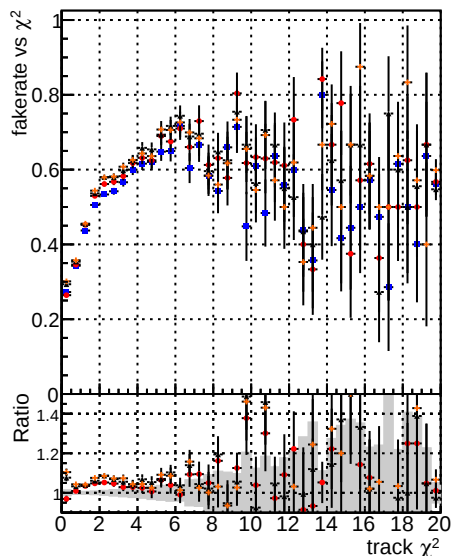
Fake rate vs. BQM mkFit T-Original 106 BQM mkFit T-NEWHSM 95 ALLITERS-106
