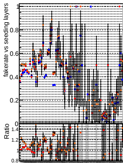
Fake rate vs. BQM mkFit T-Original 106 BQM mkFit T-NEWHSM 95 ALLITERS-106
