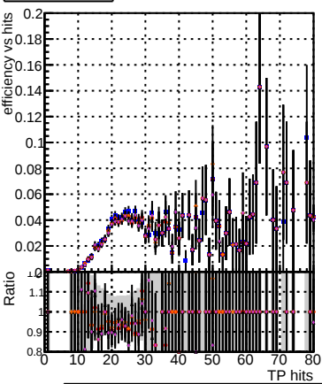
Efficiency vs hit DOM_mkFit_TToriginal DOM_mkFit_TToriginal-106 DOM_mkFit_TTNEWHSMS95_ALLITERS-106 DOM_mkFit_TTNEWHSMS95chi2_ALLITERS-106 DOM_mkFit_TTNEWHSMS95dpdq_ALLITERS-106
