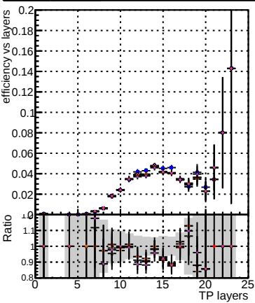
Efficiency vs hit DOM_mkFit_TToriginal DOM_mkFit_TToriginal-106 DOM_mkFit_TTNEWHSMS95_ALLITERS-106 DOM_mkFit_TTNEWHSMS95chi2_ALLITERS-106 DOM_mkFit_TTNEWHSMS95dpdq_ALLITERS-106
