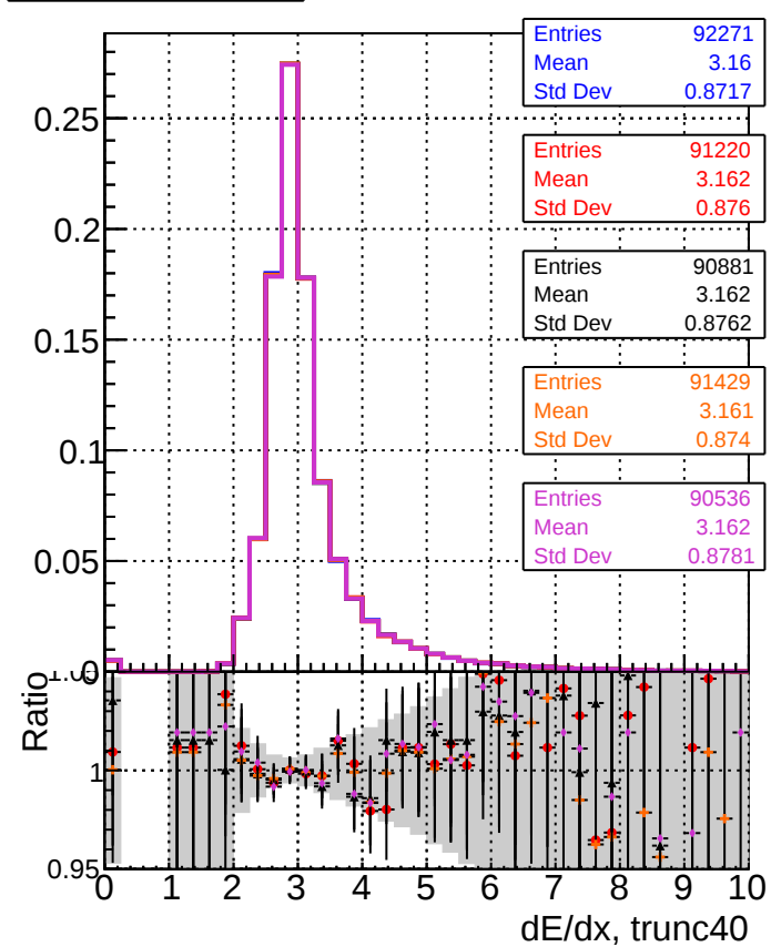
DOM_mkFit_TToriginal DOM_mkFit_TToriginal-106 DOM_mkFit_TTNEWHSMS95_ALLITERS-106 DOM_mkFit_TTNEWHSMS95chi2_ALLITERS-106 DOM_mkFit_TTNEWHSMS95dpdq_ALLITERS-106
