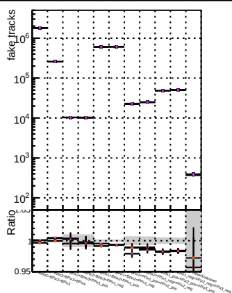
N of associated (recoToSim) fake tracks vs. \chi^2 for different filter sets
