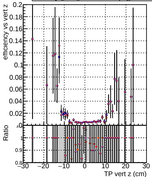
Efficiency vs TP vert z (cm) DOM mkFit Toriginal-106 DOM mkFit TNEWHSMS95 ALLITERS-106 DOM mkFit TNEWHSMS95chi2 ALLITERS-106 DOM mkFit TNEWHSMS95dpdg ALLITERS-106
