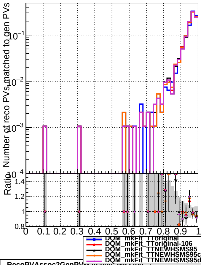
RecoPVAssoc2GenPVMatched_missing
