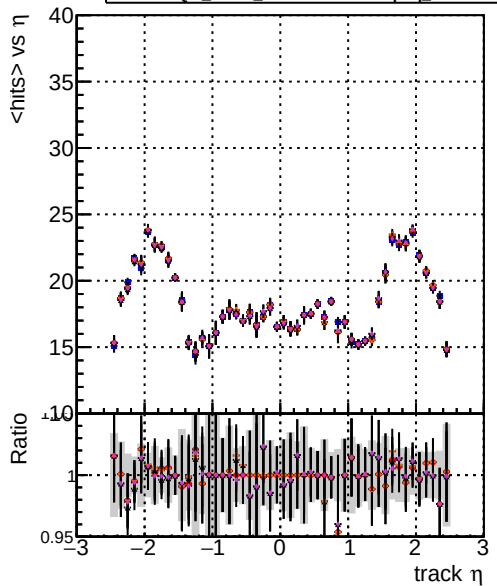
mean hit DOM mkFit Toriginal-106 DOM mkFit TNEWSMS95 ALLITERS-106 DOM mkFit TNEWSMS95ch2 ALLITERS-106 DOM mkFit TNEWSMS95dpdg ALLITERS-106
