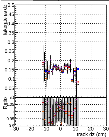
Legend for Fake rate vs d, Duplicates rate vs dz, and Pileup rate vs dz plots: DOM mkFit TToriginal TToriginal+g ALITERS-106 DOM mkFit TToriginal TToriginal+g ALITERS-106 DOM mkFit TToriginal TToriginal+g ALITERS-106
