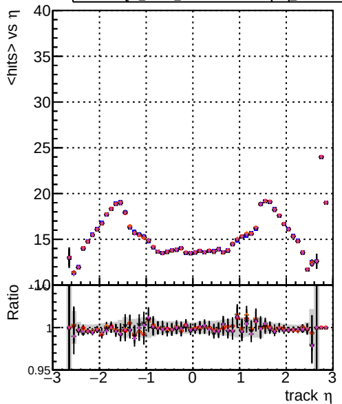
mean hits vs \eta DOM mkFit Toriginal-106 DOM mkFit TNEWHSMS95 ALLITERS-106 DOM mkFit TNEWHSMS95sch2 ALLITERS-106 DOM mkFit TNEWHSMS95dpdg ALLITERS-106
