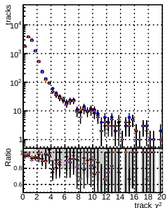
N of reco track vs. \chi^2 for different methods
