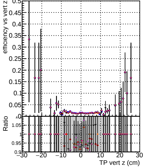
Efficiency vs. TP vert z (cm) DOM mkFit original DOM mkFit original-106 DOM mkFit NEWHSMS95 DOM mkFit ALLITERS-106 DOM mkFit NEWHSMS95ch2 DOM mkFit ALLITERS-106 DOM mkFit NEWHSMS95dpdg DOM mkFit ALLITERS-106
