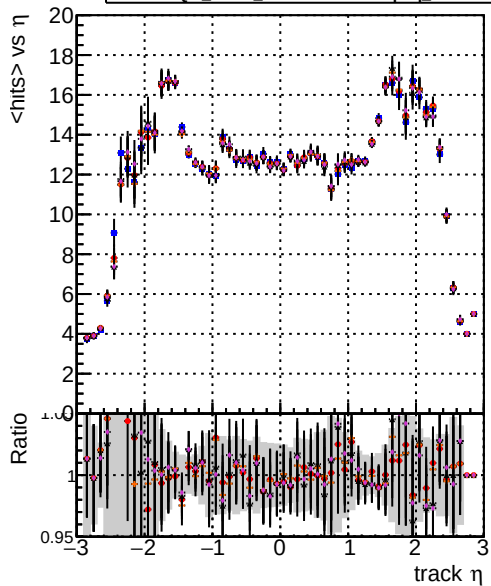
Legend for mean hits vs \eta : DOM mkFit Toriginal-106 DOM mkFit TNEWHSMS95 ALLITERS-106 DOM mkFit TNEWHSMS95ch2 ALLITERS-106 DOM mkFit TNEWHSMS95dpdg ALLITERS-106
