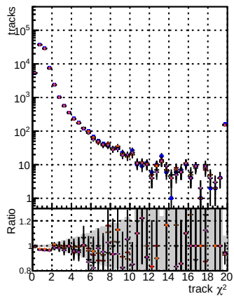
N of reco track vs. \chi^2 for BOM, mFit, TFC (original vs. ALICE-106), BOM, mFit, TFC (NEWHSN355006 vs. ALICE-106)
